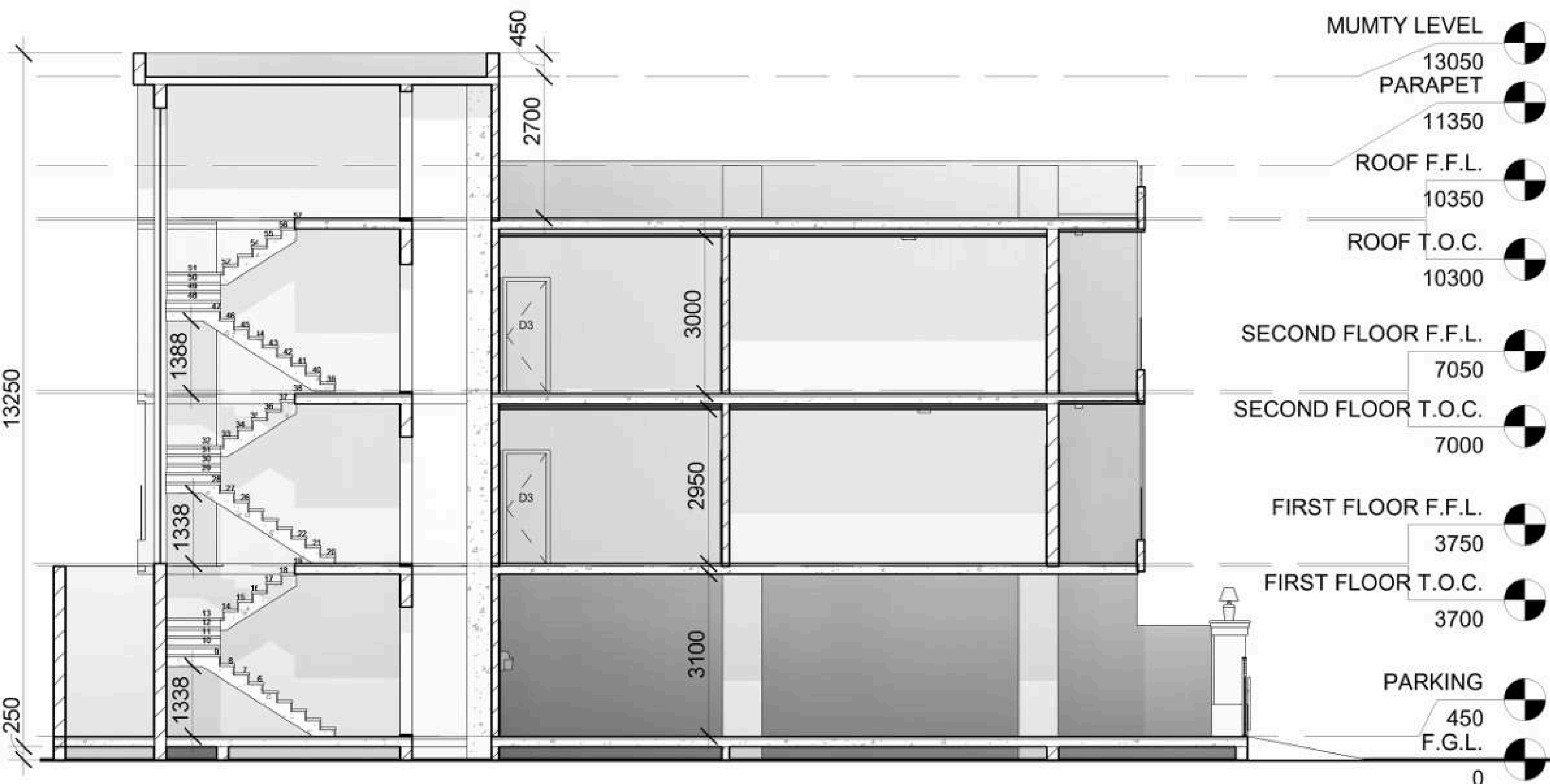
A-A SECTION VIEW
